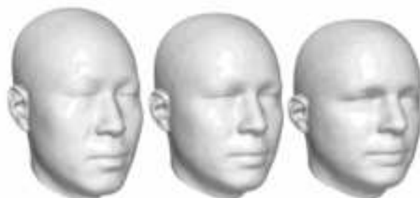
PC4
